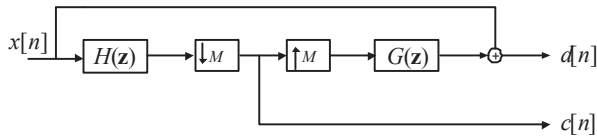
Fig. 1. Implementation of the LP frame.
