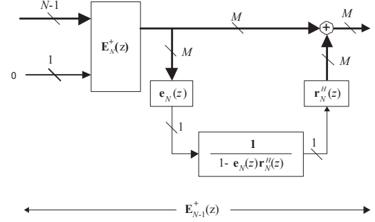
Fig. 2. Post-filtering based implementation structure for \mathbf{E}_{N-1}^\dagger(z)
