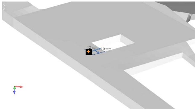
Figure 6-20. Joint probe location on FEM (orange star).
