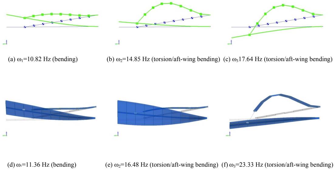
Figure 4-6. Natural modes of beam strut (a-c) and wingbox (d-f) models where fore and aft wings optimized separately to match natural frequencies and mode shapes.
