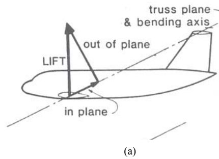
Fig. 5 Tilted bending axis of a joined wing
