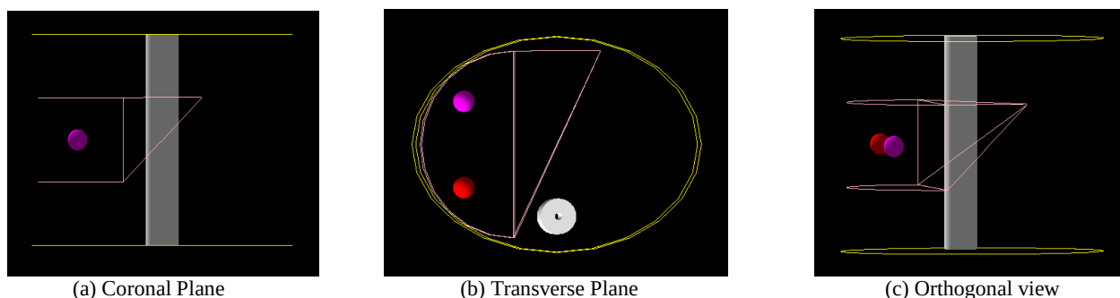
Figure 3. GEANT4 simulation of the liver iron overload sample. The outline of the torso is marked by the yellow lines. The liver is shown as a pink outline with two high concentration spherical lesions inside. Each lesion contains a different concentration of iron. The spine is visible as a white cylindrical tube. (Figure from [12]).
