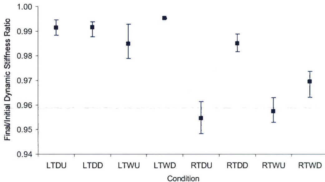
Figure 9. Ratio of final to initial dynamic stiffness as a function of test conditions.
