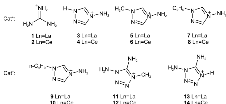
Scheme 1. Ionic liquids based on lanthanide nitrate complex anions
