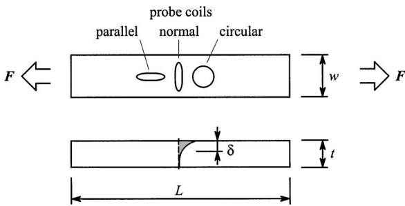
Fig. 3. A schematic diagram of the experimental arrangement used to measure electro-elastic coefficients in uniaxial compression and tension.
