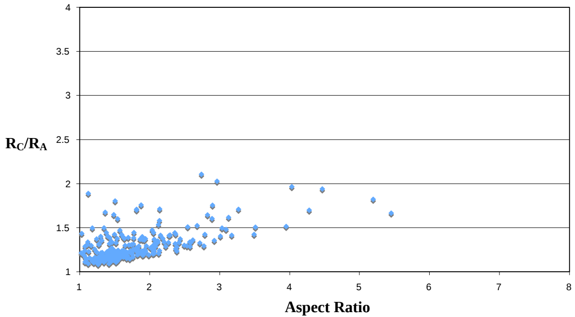
FIGURE 5 - Distribution of 144 to 177 µm Commercially Available Foundry Sand Sample
