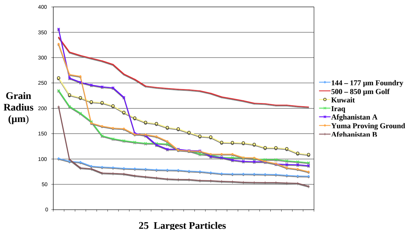
FIGURE 20 – Grain Size Distribution of 25 Largest Particles from Sand Samples
