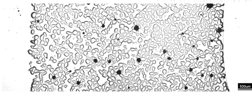
FIGURE 6 - Reflected Light Image of 144 to 177 µm Commercially Available Foundry Sand Sample
