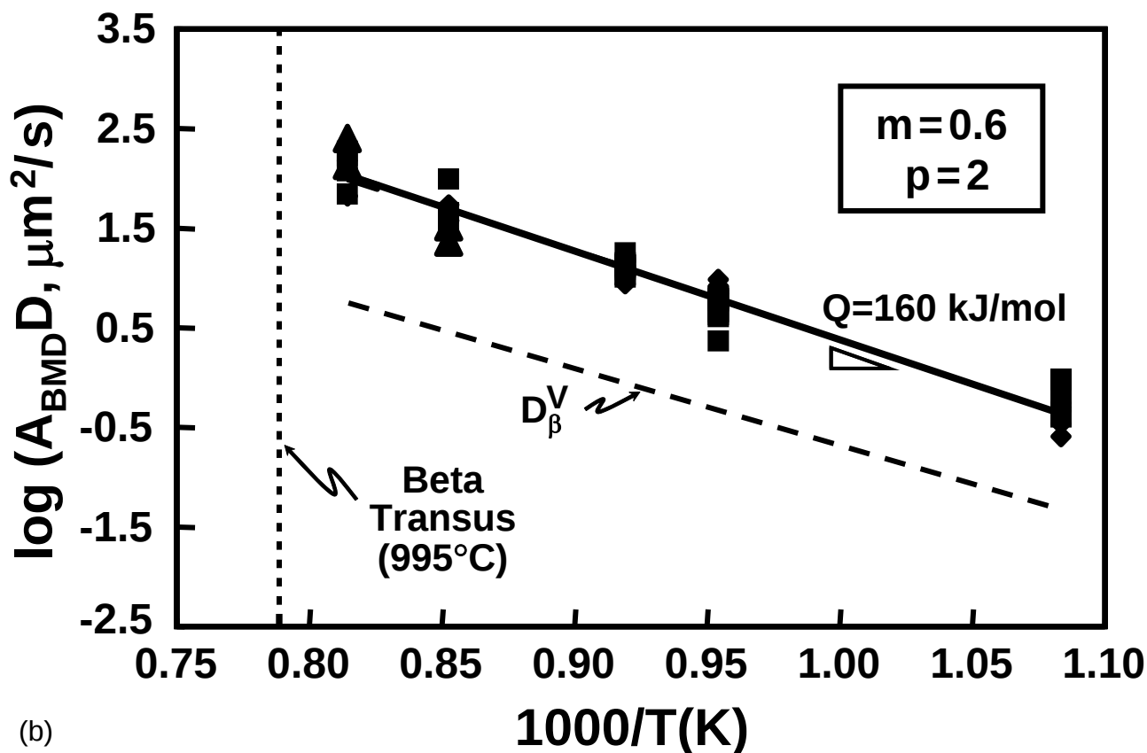
Figure 10. Effect of dynamic coarsening on plastic flow of Ti-6Al-4V with an equiaxed- \alpha microstructure [40]: (a) selected flow curves and (b) constitutive analysis to determine the appropriate activation energy and diffusivity to describe superplastic flow.
