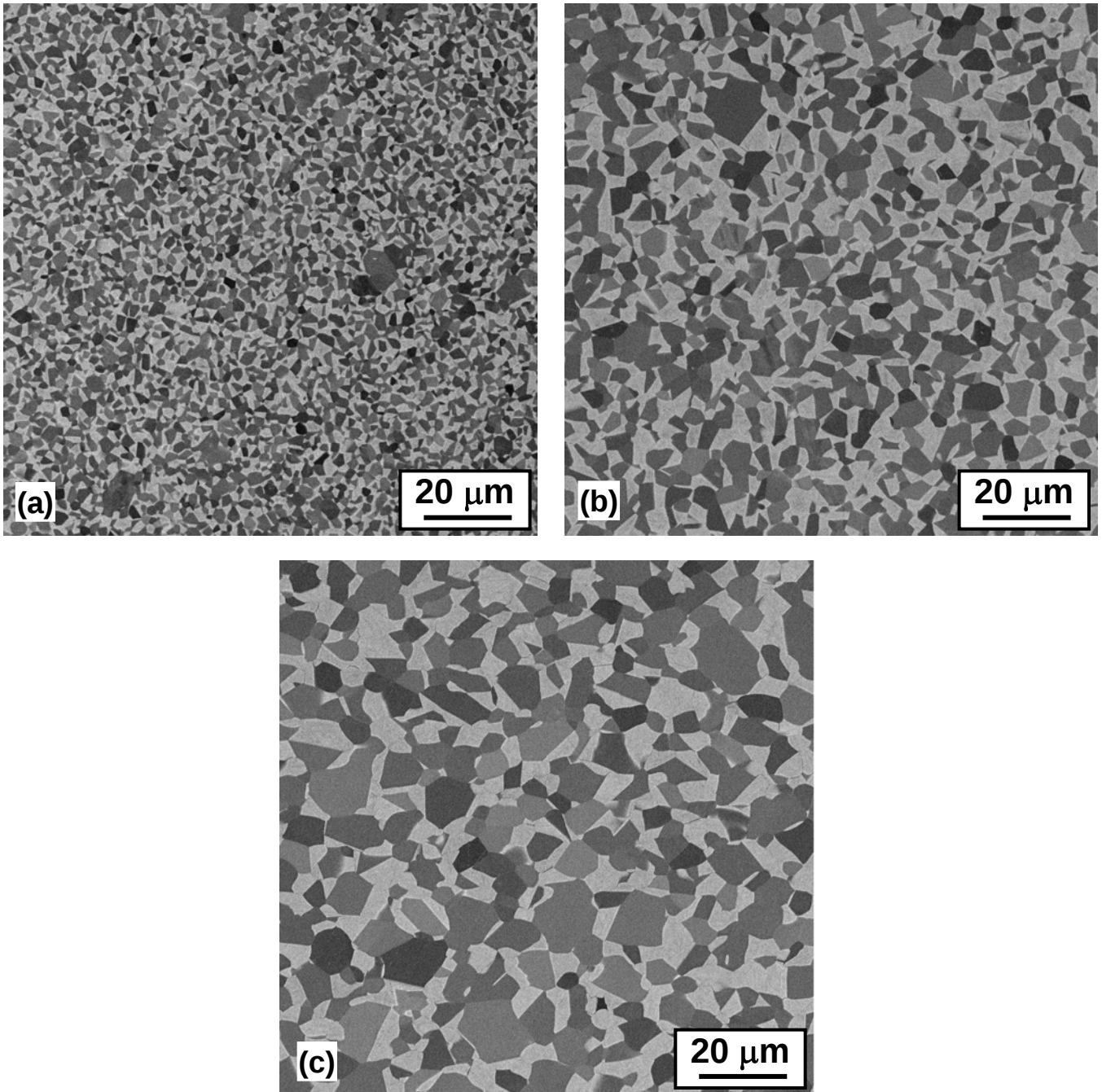
Figure 9. SEM backscattered micrographs taken at the same magnification illustrating dynamic coarsening of Ti-6Al-4V samples with an equiaxed-alpha microstructure deformed at 900°C, 10^{-4} \text{ s}^{-1} to true strains of (a) 0, (b) 0.5, and (c) 1.4, followed by water quenching [42]. The compression axis is vertical for each micrograph. (Alpha ~ darker phase, beta ~ lighter phase)
