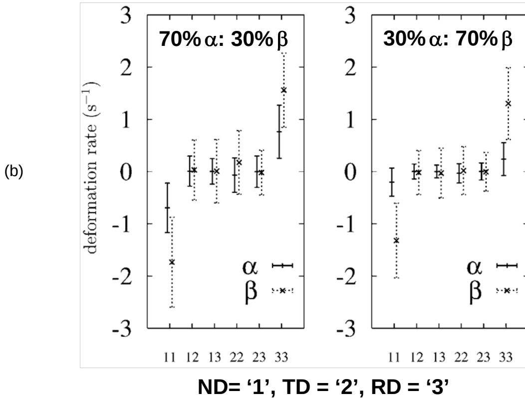
Figure 21. Strain partitioning in two-phase alloys: (a) Comparison of CPFEM meso-scale and micro-scale model predictions with those from a self-consistent model [62] and (b) CPFEM predictions of the strain components in the alpha and beta phases during rolling of titanium plate with two different volume-fraction ratios [63].
