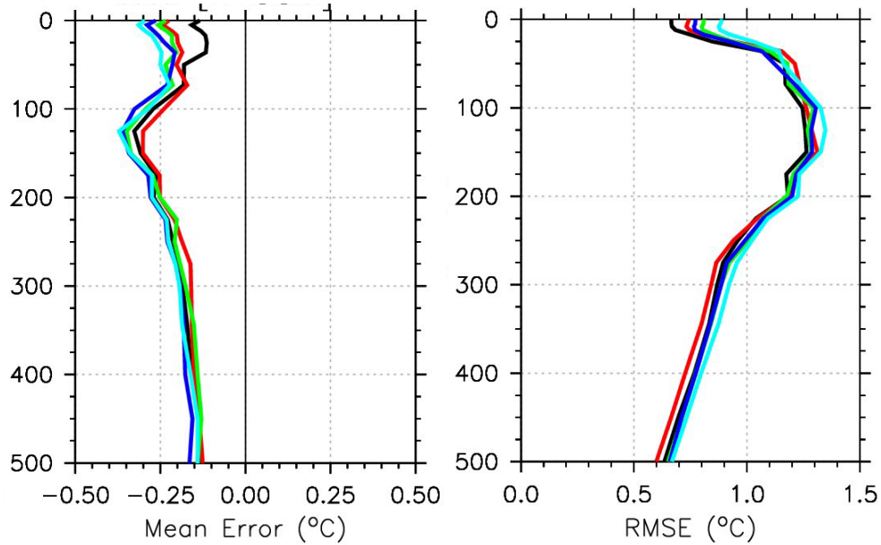
Figure 24: Temperature (°C) vs. depth error analysis in the upper 500 m of the near-global MERall region for Spring (MAM) 2008 using 3874 unassimilated profiles. The left panel is mean error and the right panel is RMSE. The lines represent the error associated with an n-day forecast from the initial state of the hindcast: black = 1-day forecast, red = 2-day forecast, green = 3-day forecast, blue = 4-day forecast and cyan = 5-day forecast.
