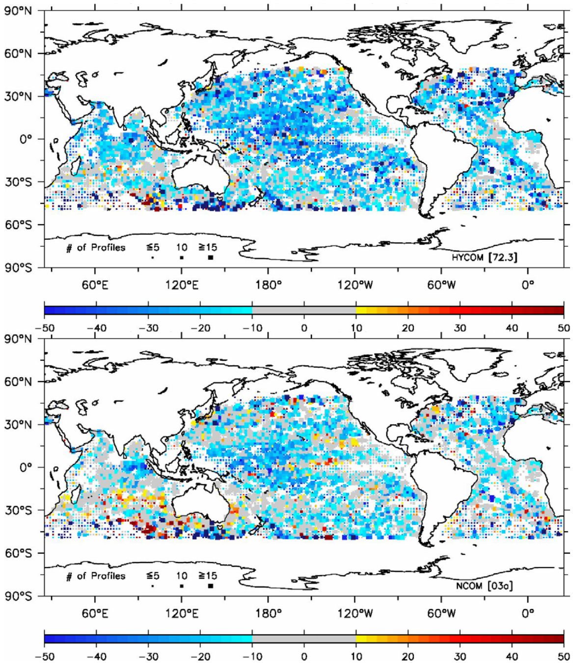
Figure 30: As in Figure 28 except for SLD and the number of unassimilated profiles is 50681. For V3.0, the basin average MdBE = -16 m, RMSE = 67 m and 25% of the points are within 10 m of the observation. For V2.5, the basin average MdBE = -10 m, RMSE = 60 m and 34% of the points are within 10 m of the observation.
