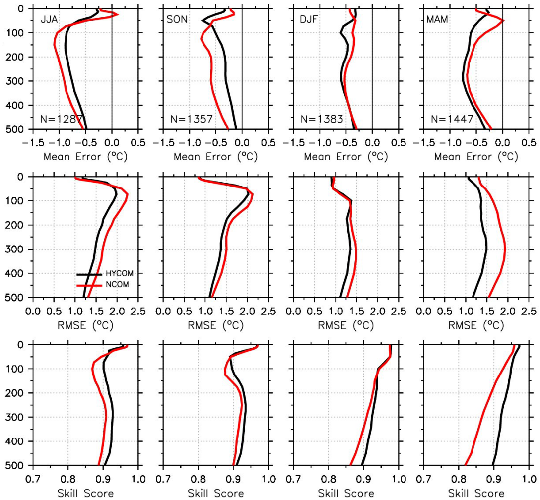
Figure 18: As in Figure 16 except for the western Pacific region (120-170°E, 20-50°N). Note the scales on the x-axes of the ME and RMSE panels are different than those on Figure 16.
