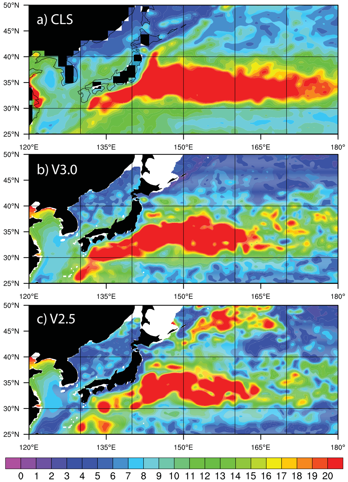
Figure 9: As in Figure 7 except for the Kuroshio region.
