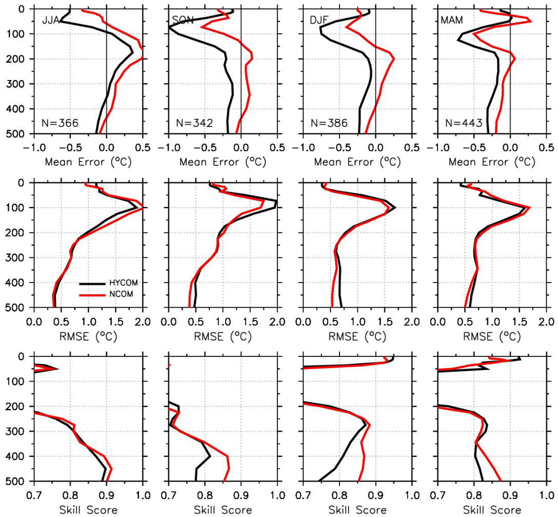
Figure 19: As in Figure 16 except for the Arabian Sea region (45-80°E, 0-24°N).
