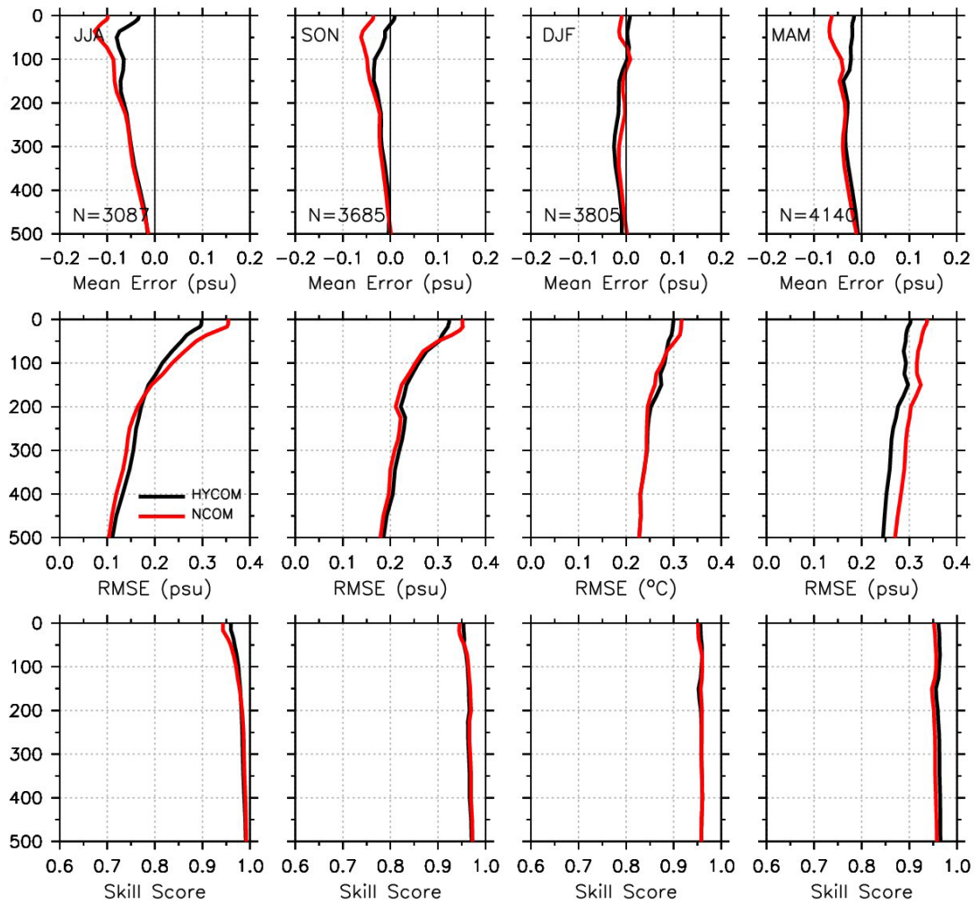
Figure 21: As in Figure 20 except for the MER4d region.
