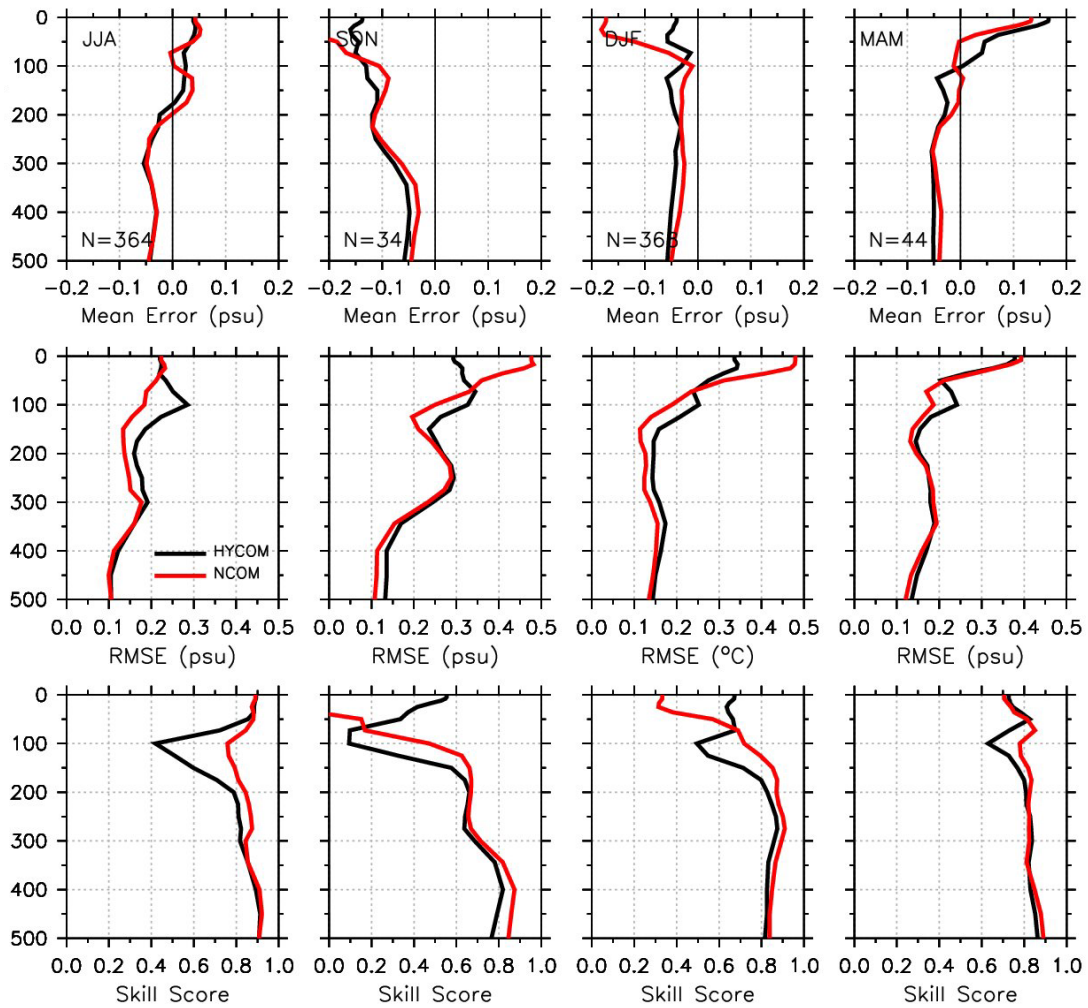
Figure 23: As in Figure 20 except for the Arabian Sea region (45-80°E, 0-24°N). Note that the range of the x-axes for RMSE and SS is different than that for Figure 20.
