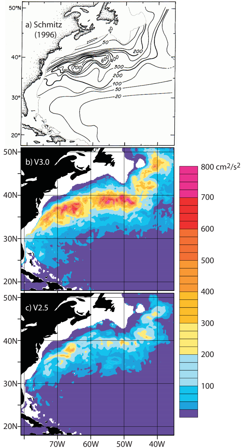
Figure 12: EKE (cm 2 /s 2 ) for the Gulf Stream region at 700 m depth from a) Schmitz (1996), b) GOPS V3.0 and c) GOPS V2.5. The observations are compiled from SOFAR float observations. The simulated results span the hindcast time frame, 1 June 2007 – 31 May 2008.
