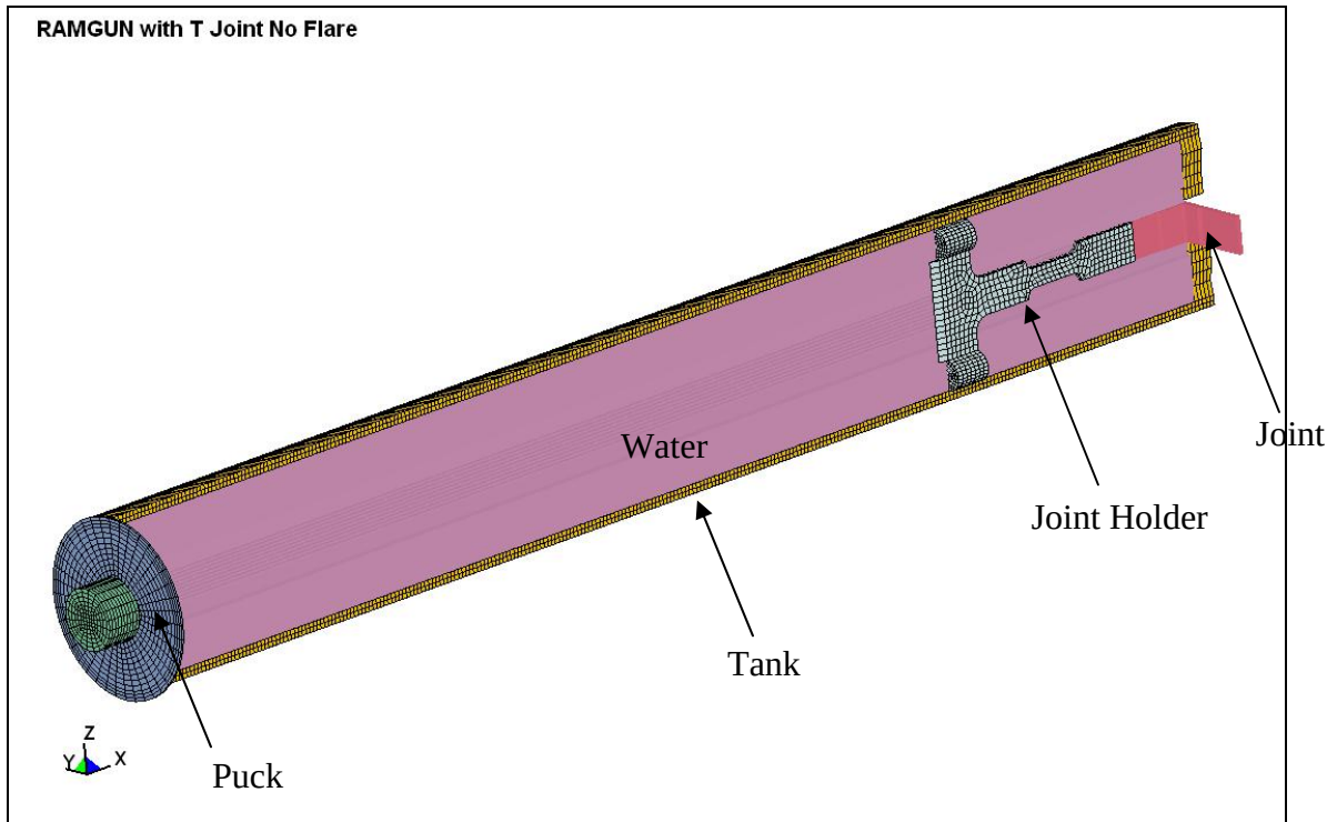
Figure 2.4-3 LSDYNA Model of Hydrodynamic Ram Simulator with no Flare and Joint ( 1.0 \times D )
