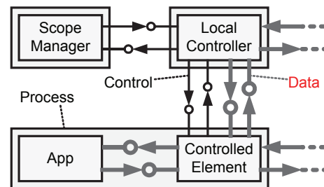
Figure 20. The architecture of a leaf scope in the most general scenario, with a local scope manager, a thin controlled element linked to the application, and with a local controller to handle peer-to-peer aspects, for example, forwarding
