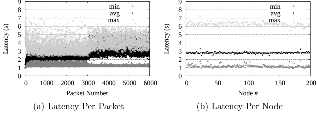
Fig. 11. Latency of packets on Emulab
