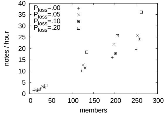
Figure 6: Number of notes sent per correct member per hour as a function of the number of members for various P_{loss} .
