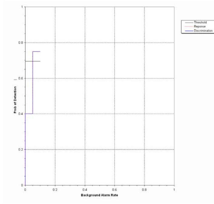
Figure 3. EM61/towed array open field probability of detection for response and discrimination stages versus their respective background alarm rate over all ordnance categories combined.
