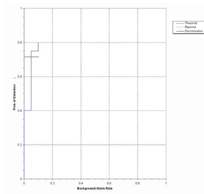
Figure 5. EM61/towed array open field probability of detection for response and discrimination stages versus their respective background alarm rate for all ordnance larger than 20 mm.
