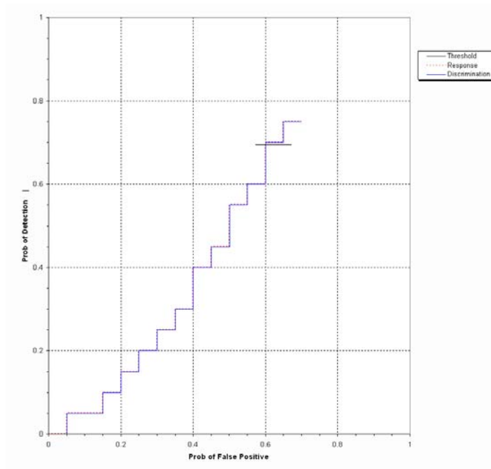
Figure 2. EM61/towed array open field probability of detection for response and discrimination stages versus their respective probability of false positive over all ordnance categories combined.
