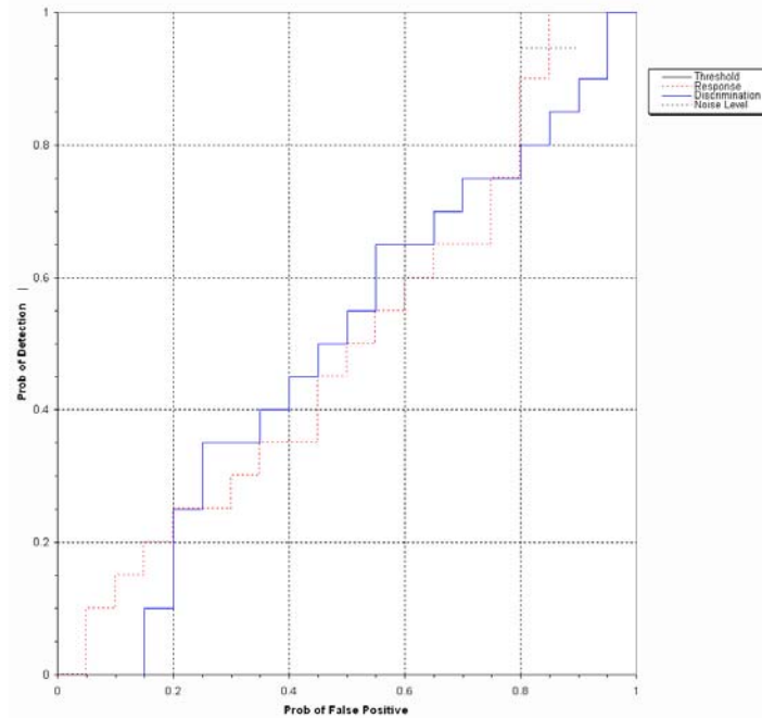
Figure 8. EM61 MKII/towed array P_d^{\text{res}} versus the respective P_{\text{fp}} for ordnance larger than 20 mm.
