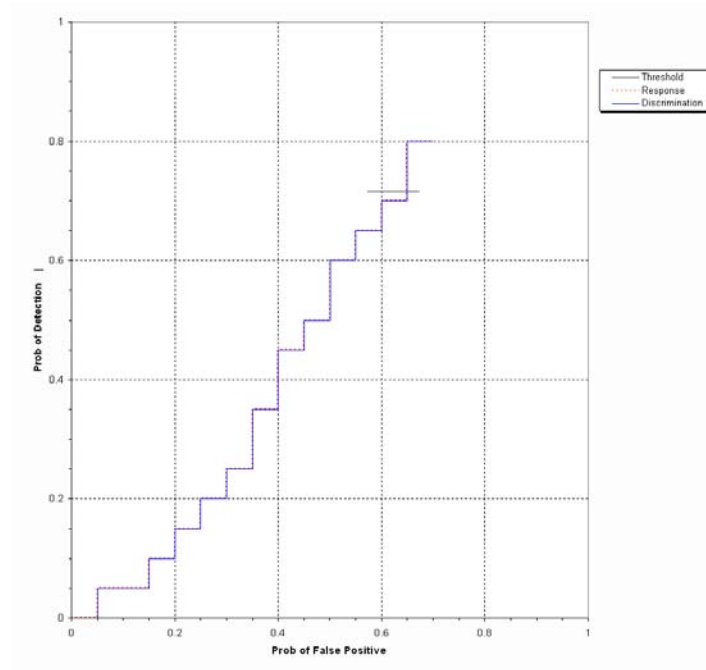
Figure 4. EM61/towed array open field probability of detection for response and discrimination stages versus their respective probability of false positive for all ordnance larger than 20 mm.
