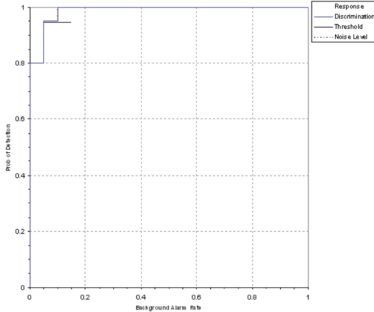
Figure 9. EM61 MKII/towed array P_d^{\text{disc}} versus the respective P_{\text{fp}} for ordnance larger than 20 mm.
