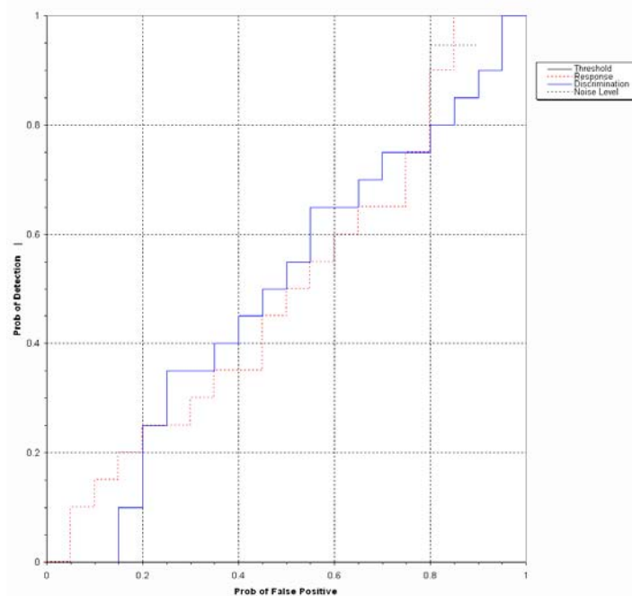
Figure 4. EM61 MKII/towed array blind grid probability of detection for response and discrimination stages versus their respective probability of false positive for all ordnance larger than 20 mm.
