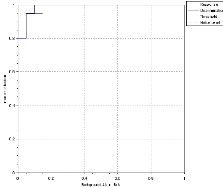
Figure 3. EM61 MKII/towed array blind grid probability of detection for response and discrimination stages versus their respective background alarm rate over all ordnance categories combined.
