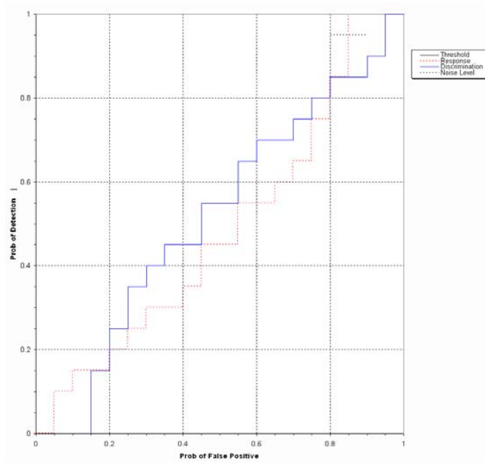
Figure 2. EM61 MKII/towed array blind grid probability of detection for response and discrimination stages versus their respective probability of false positive over all ordnance categories combined.
