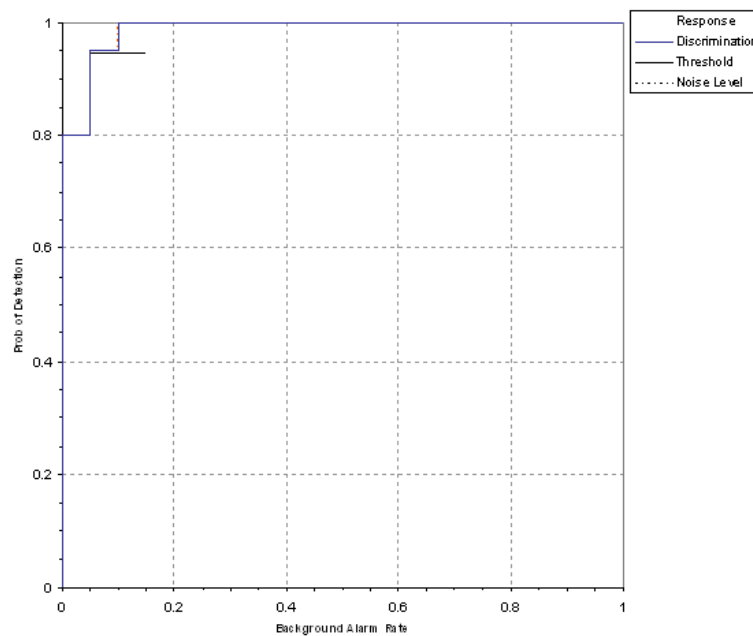
Figure 5. EM61 MKII/towed array blind grid probability of detection for response and discrimination stages versus their respective background alarm rate for all ordnance larger than 20 mm.
