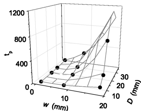
FIG. 15. The variation in the time to the peak electron current t_p arriving at the anode with the hollow cathode depth, D , and thickness, w , and the seed electrons are injected with no mean velocity and a temperature of 2.5 eV. The grid is a best fit to the data.
