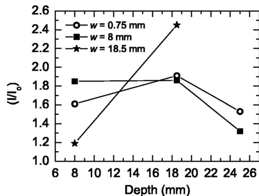
FIG. 16. The variation in the peak electron current arriving at the anode with the hollow cathode depth, D , and thickness, w , where I_0 is the peak current for D=8 mm, w=0.75 mm, h=8 mm and 1 keV seed electrons, the hole height h=8 mm, and the seed electrons are injected with an average energy equal to the ionization peak.
