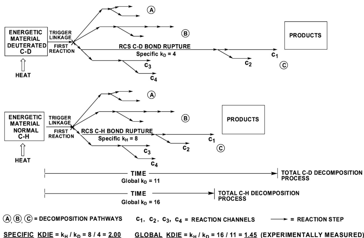
Fig. 1. General thermochemical decomposition process schematic representation and the KDIE measurement context [13].
