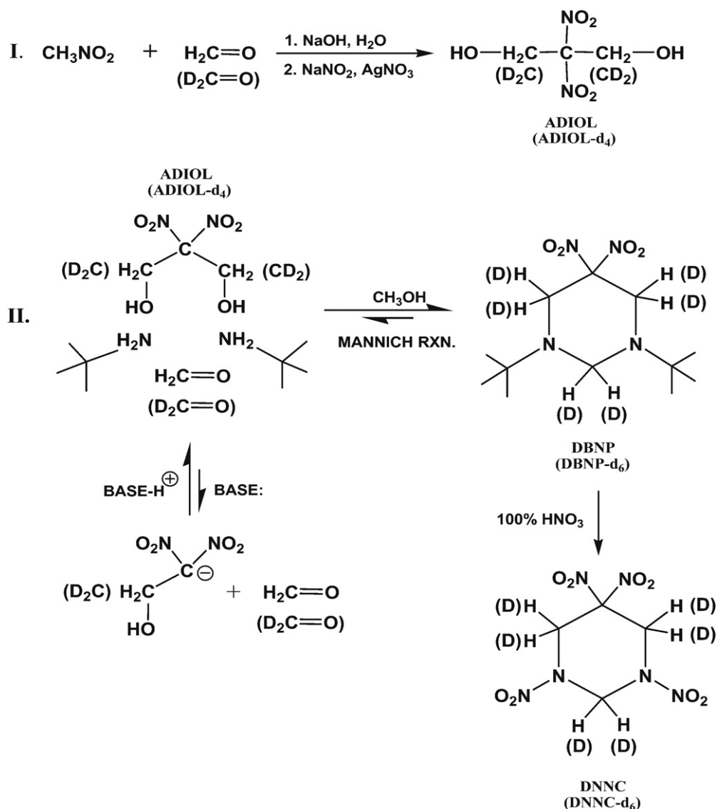
Fig. 11. General synthesis scheme used for ADIOL, ADIOL- \text{d}_4 and the four DNNC isotopomers.
