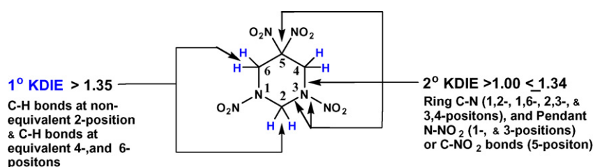
Fig. 8. Possible KDIE types from C–H (1° KDIE) bond rupture and C–N, N–NO 2 , C–NO 2 (2° KDIE) potentially present with the DNNC molecular structure.
