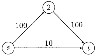
Figure 1. Interdiction decisions based on expected residual arc capacities may be incorrect.
