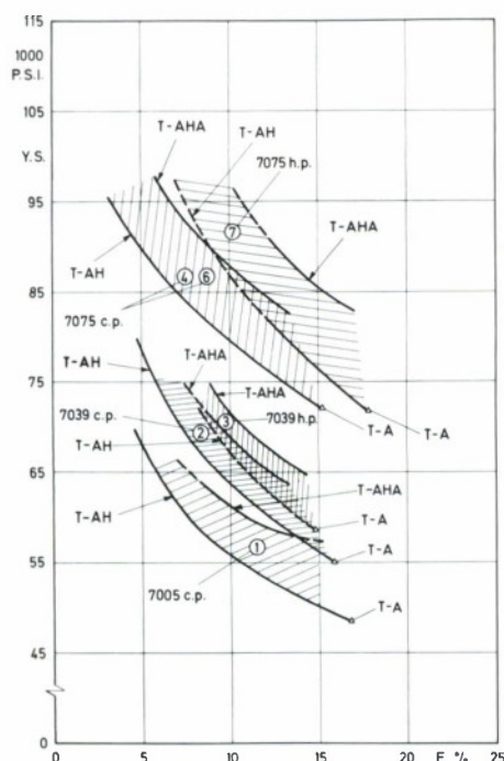
Fig. 4—Yield strength values vs elongation of sheets of 7005, 7039, and 7075 alloys in several thermal and thermomechanical tempers.
