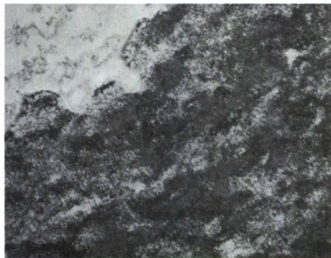
Fig. 8—Transmission electron micrograph of 2 mm-thick sheet of 7075 h.p. alloy (No. 7) in T-H10 pct A120°C for 24 h temper. Magnification 19,200 times.
