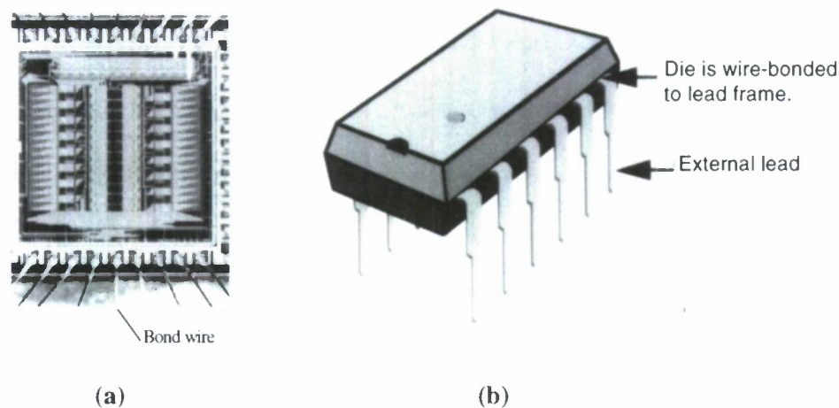
Figure 2.1 Major components of an integrated circuit (a) Die and bond wires connecting die to external leads (b) Plastic-molded dual-in-line package
