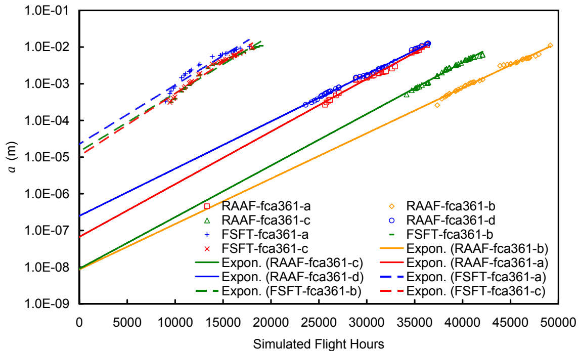
Figure 6: Exponential extrapolation to evaluate a_0
