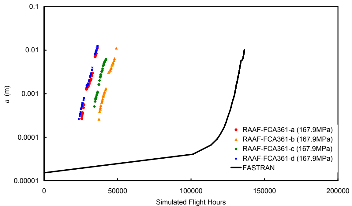
Figure 14: FASTRAN prediction for the RAAF spectrum using an initial crack size of 1.52 \times 10^{-5} \text{ m} compared to the RAAF coupon data
