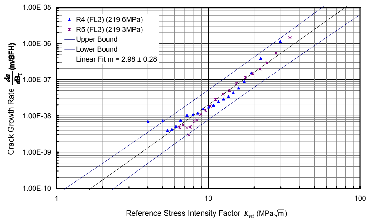
Figure 26: Crack growth rate data obtained from QF coupons subjected to the FL3 spectrum
