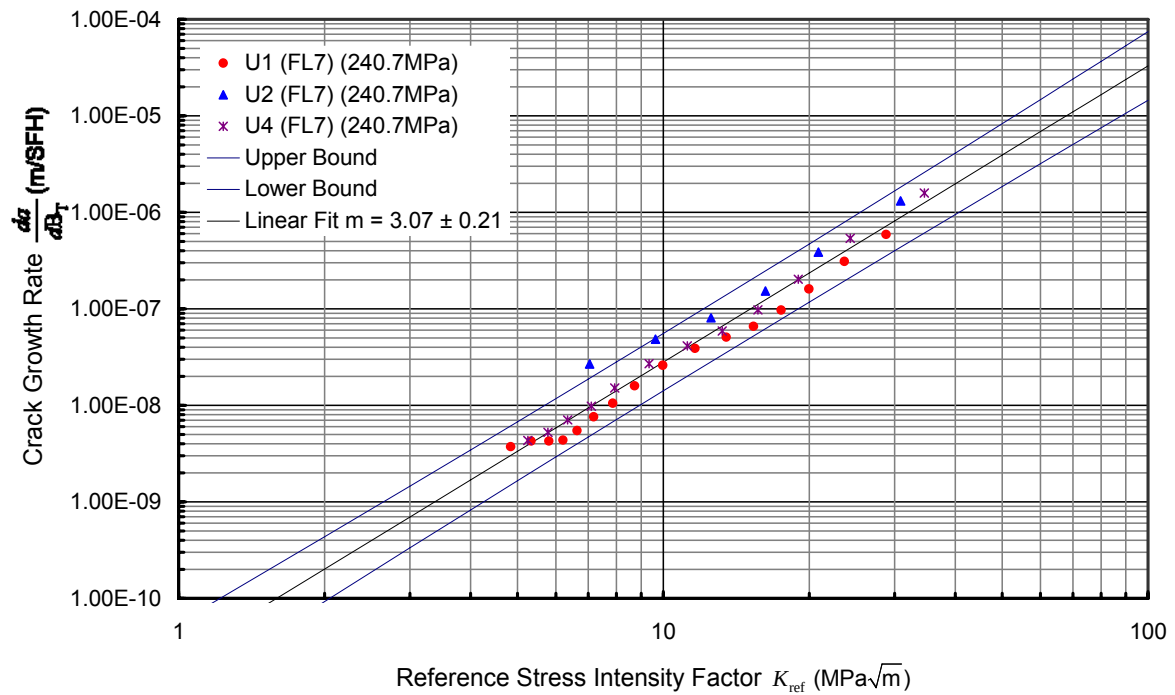
Figure 32: Crack growth rate data obtained from QF coupons subjected to the FL7 spectrum
