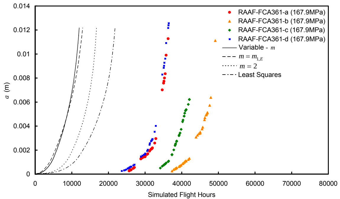
Figure 13: EBA prediction for the RAAF spectrum using an initial crack size of 1.52 \times 10^{-5} \text{ m} compared to the RAAF coupon data
