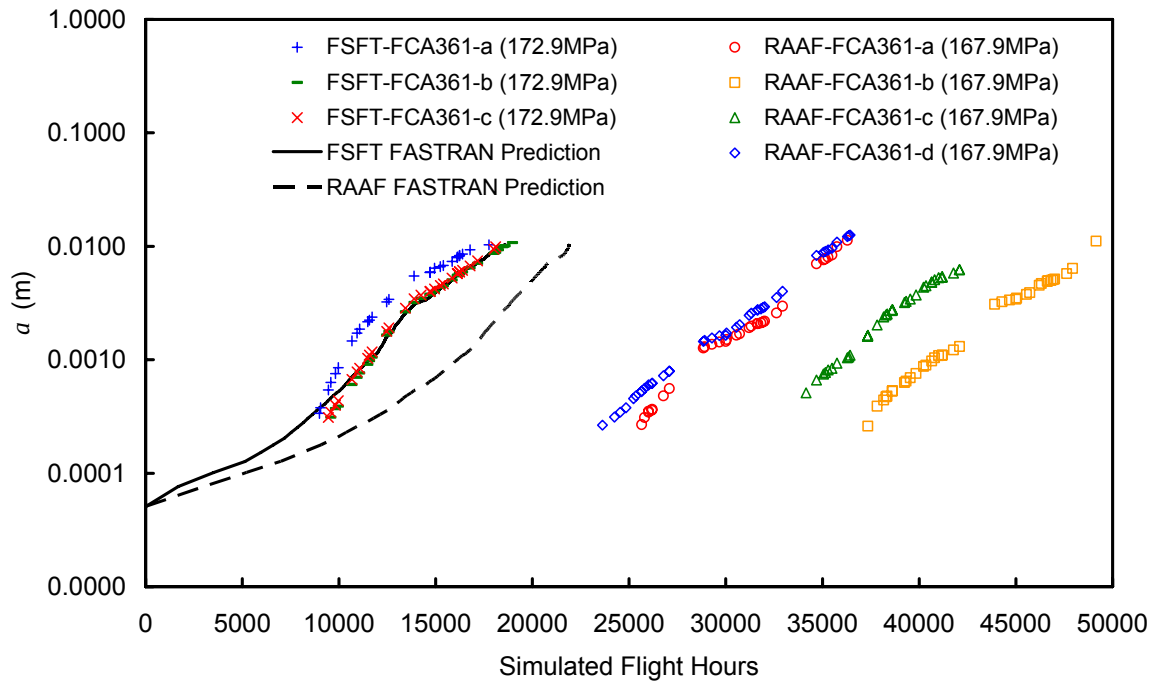
Figure 8: FASTRAN Predictions for FSFT and RAAF spectra, a_0=0.05 mm
