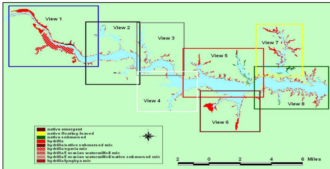
Figure B1. Lake Gaston, NC/VA, Views 1 – 8, September 2005 SOG Survey Maps.
