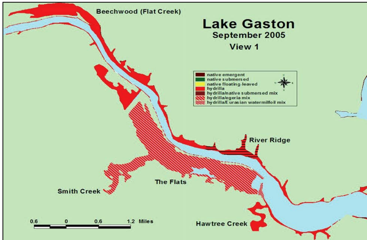
Figure B2. Lake Gaston, NC/VA, View 1, September 2005 SOG Survey Maps.
