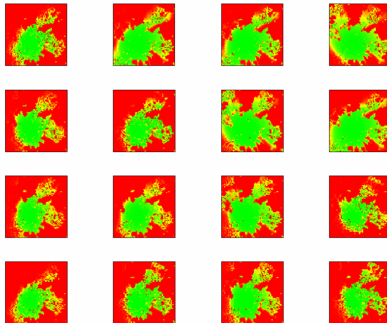
Figure 10. Probability of detection calculations based on 16 random combinations of source height, noise background, ground permeability, wind speed, and wind direction. The individual plots correspond to an overhead view of the probability of detection as in Figure 5 (right), with the horizontal coordinate being the easting and vertical being the northing.
