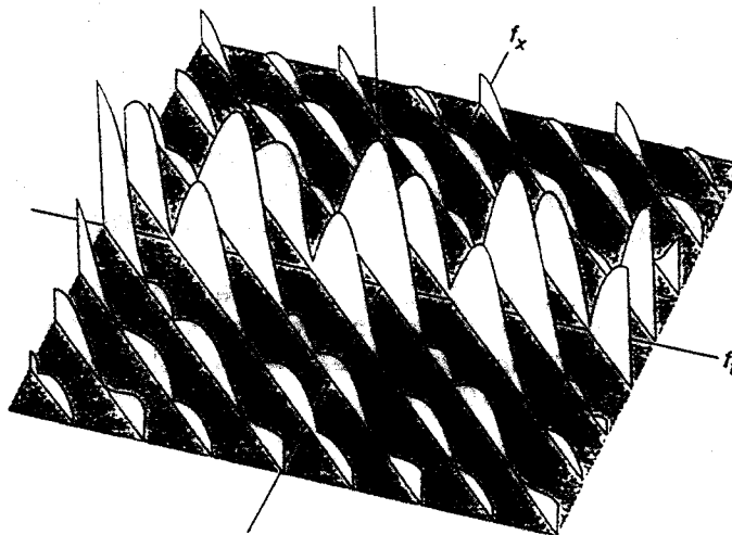
Figure 1. Image Spectra
