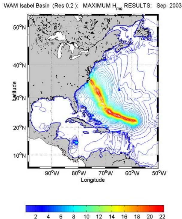
Figure 1: Maximum wave heights along Isabel's path generated by WAM-4.
