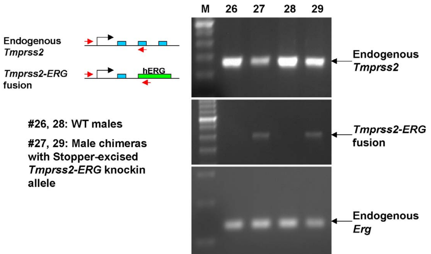
Figure 1. Expression of the Tmprss2-ERG fusion transcript from the Stopper-excised Tmprss2-ERG knockin allele (thus activated) determined by RT-PCR. PCR primers used to detect the endogenous Tmprss2 transcript and the Tmprss2-ERG fusion transcript are shown in the schematic drawing (red arrows). PCR primers used to detect the endogenous mouse Erg are located in exons further downstream (not shown).
