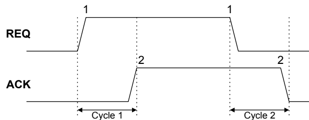
Figure 23. Asynchronous Two-phase Handshaking Model
