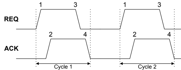
Figure 24. Asynchronous Four-phase Handshaking Model
