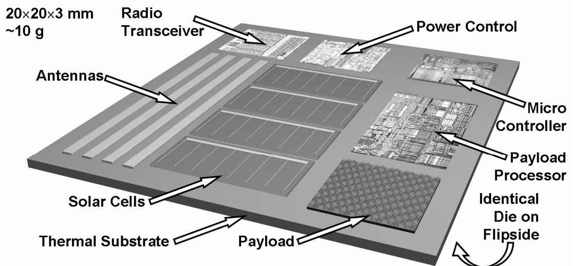
Figure 4. Notional System Configuration
