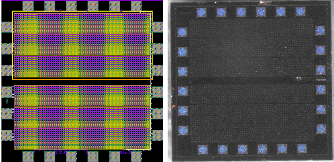
Figure 11. Cadence Layout and Die Micrograph of Solar Cell Test Chip #1
