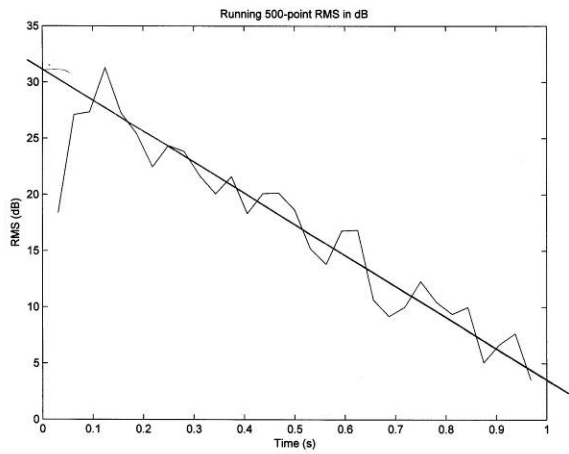
Figure B-3. RMS values on log scale as a function of linear time, with straight-line fit to estimate decay rate. Octave-band samples with center frequencies 125, 250 and 500 Hz (left column) and 1000, 2000 and 4000 Hz (right column). Samples were measured before installation of additional acoustics panels. Third sample set.
