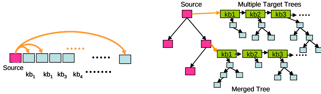
Figure 8. Representing the knowledge base using merged tree.
