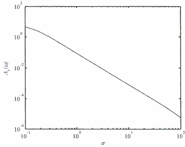
Figure 11: The spectrum of the gust \Lambda_v(\omega) = |\tilde{v}(\omega)U / a\Delta v|^2 used for the calculation of lift spectra as a function of reduced frequency \sigma .
