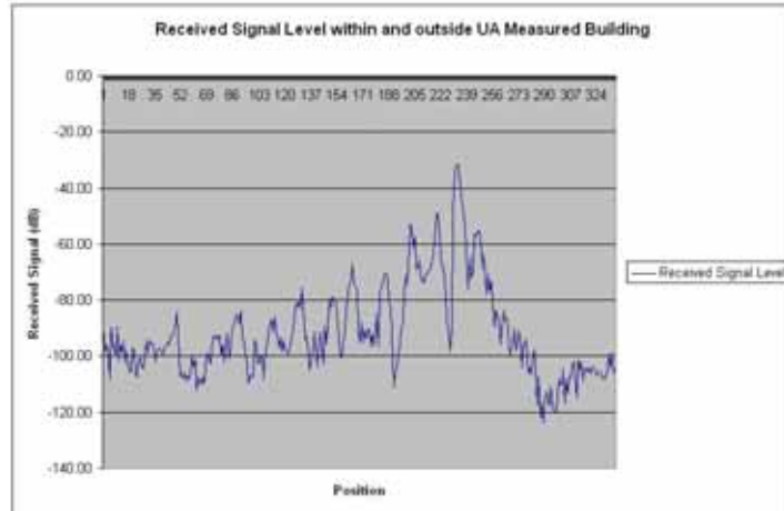
Figure 22. Normalized received signal level (negative path loss) in dB within and outside the measured building at the University of Arizona. The transmitter was on the ground floor and operating at 49 MHz.
