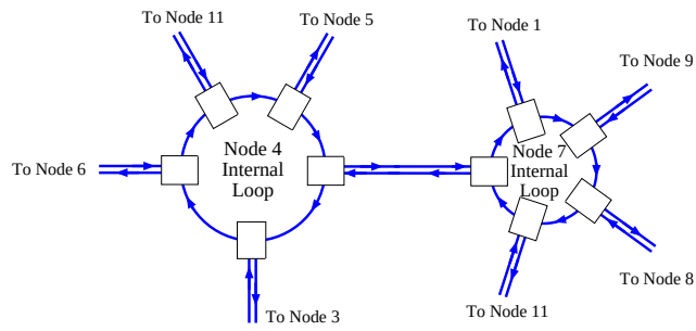
Figure 11: Example internal loops. The loops shown correspond to those of nodes 4 and 7 from the example of Figure 10. Links unnecessary to recovery are excluded from the internal loops.
