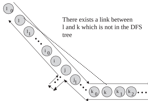
Figure 6: Collection route before link failure.
