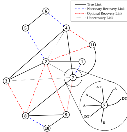
Figure 10: Example DFS tree and labeling. The graph shown is the NJ LATA network. An expanded version of node 7 is labeled with ancestor (A), descendant (D), and tree (T) markings. Link styles indicate their relevance to the collection route and recovery.
