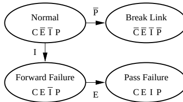
Figure 13: State diagram for an AT link device.
