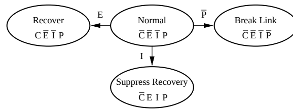
Figure 16: State diagram for a D link device.
