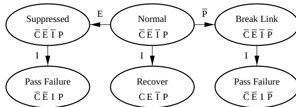
Figure 14: State diagram for a DT link device.
