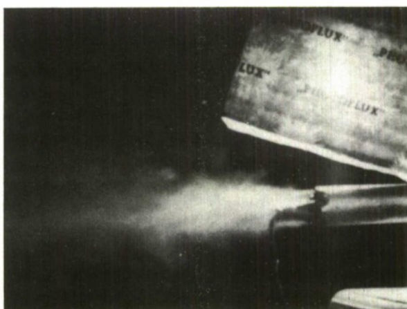
BURN THROUGH OF STEEL CAP 0.200 sec. AFTER FIRING
