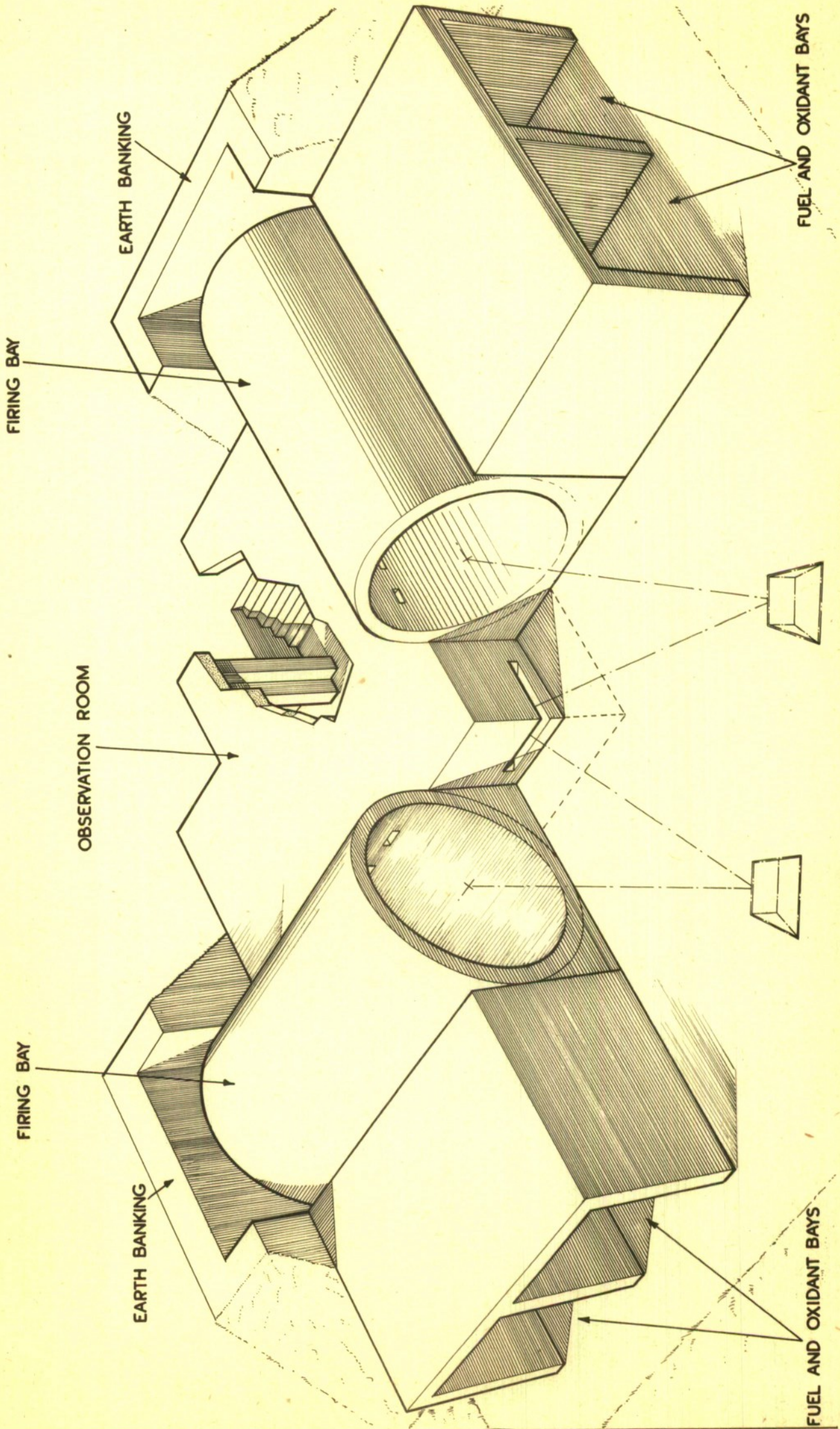
FIG.2. FIRST DESIGN OF TWIN EMPACEMENT
