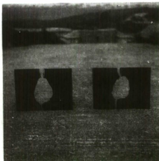
Photo No. 7. The 5/16" plate holed and broken
