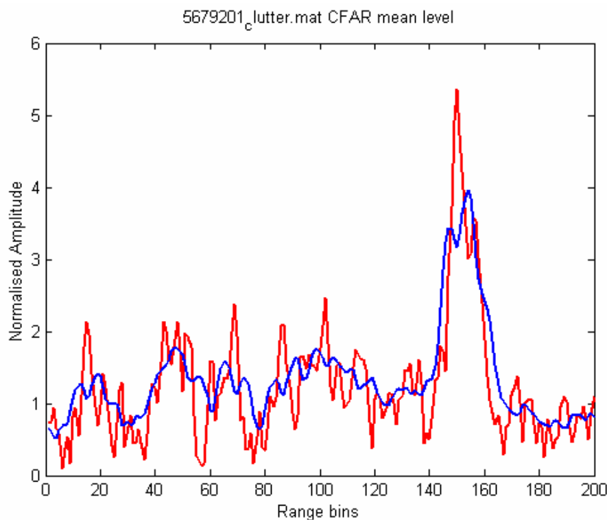
Figure 21: Variation of mean clutter plus noise estimate with range in strongly correlated K-distributed clutter ( R_{cor}=10 ) (red – clutter plus noise mixture range profile; blue - mean clutter plus noise level estimate for a double-sided CA CFAR with N=5 and G=1 ).
