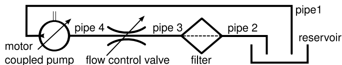
Fig. 1. The diagram representing the simplified pump system.
