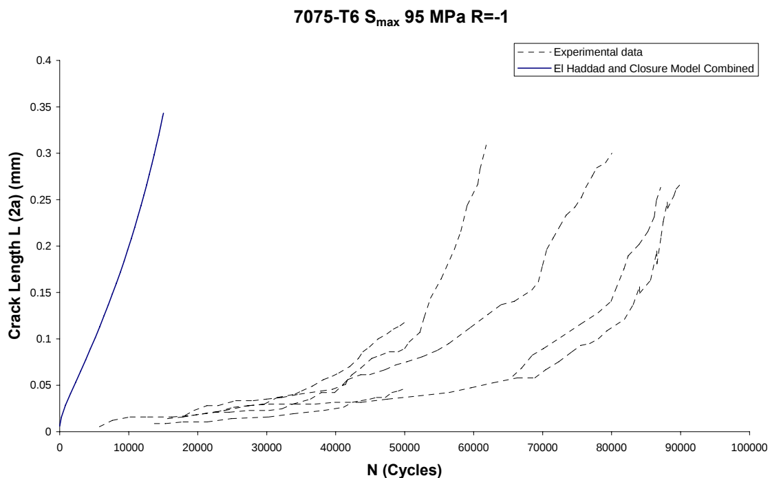
Figure 23: Crack growth comparison, experimental data compared with CGAP results obtained by activating both the FASTRAN model and the El Haddad model with a_0 = 0.086 mm 7075-T6 alloy S_{max} = 95 MPa R = -1
