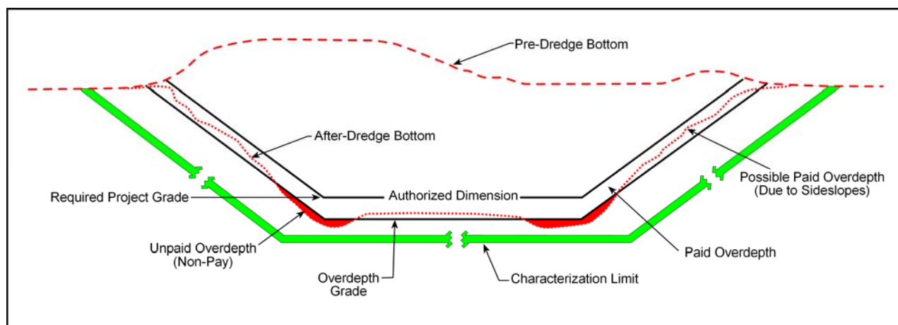
Figure 2.3-4 Various Dredging Prism Dimensions and Zones
