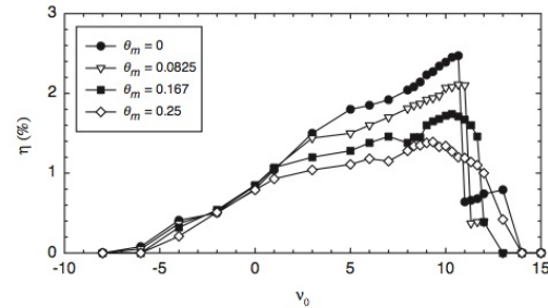
Fig. 3. Efficiency \eta vs. initial phase velocity v_0 for several mirror tilts \theta_m for the 1 MW simulations. Actual mirror tilt is (0.728 \text{ mrad})\theta_m .
