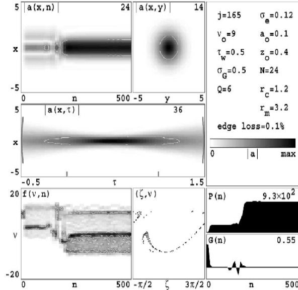
Fig. 3. Three dimensional simulation in x , y , and \tau over many passes n , for normalized Rayleigh length z_0 = 0.4 .
