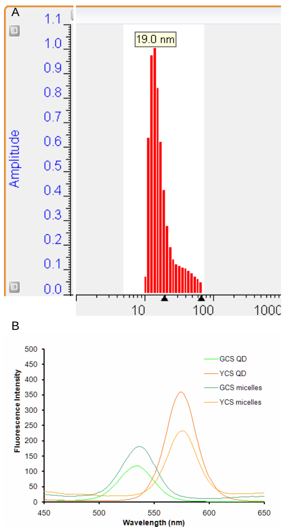
Figure 9. Characterization of quantum dot containing micelles. (A) Dynamic light scattering showing typical size distribution of YCS quantum dot micelles. (B) Fluorescent spectrum showing fluorescence emission for quantum dots before and after micelle formation. Excitation was performed at 350 nm.
