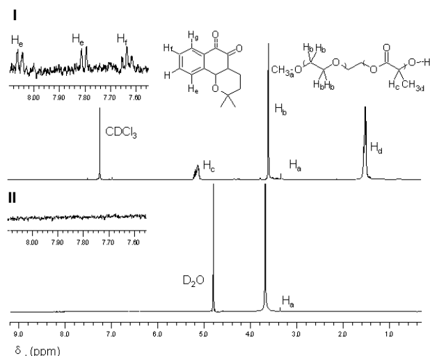
Figure 2. ^1\text{H} -NMR spectra of \beta -lap-loaded PEG-PLA micelles in (I) deuterated chloroform ( \text{CDCl}_3 ) and (II) deuterated water ( \text{D}_2\text{O} ). Figure insets represent magnifications of the aromatic protons from \beta -lap.
