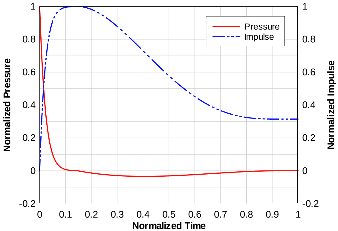
Fig. 4.4. SBEDS predicted load for Detonation 3
