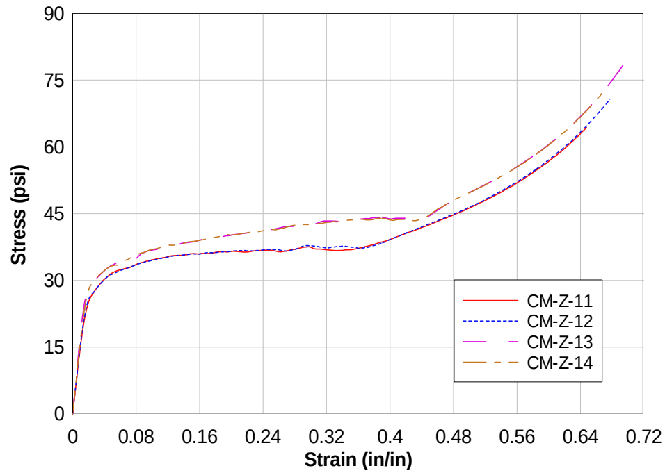
Fig. 3.7. Stress-strain behavior of Pactiv XEPS foam
