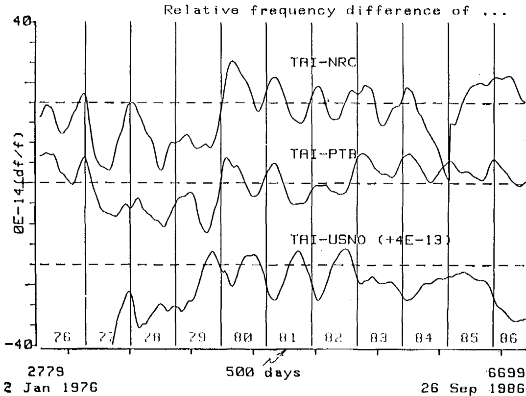
Figure 1. The relative frequency differences between TAI and the time scales of NRC, PTB and USNO. For each curve the dotted line is TAI.
