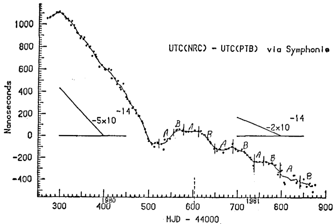
Figure 2. The difference between the UTC time scales of NRC and PTB as measured by two-way time transfer via the Symphonie satellite.
