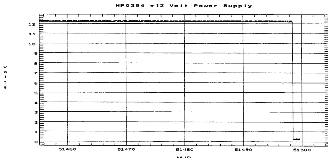
Figure 5. A performance affecting drop in the +12 volt power supply in an HP 5071 Cesium-Beam Frequency Standard.
