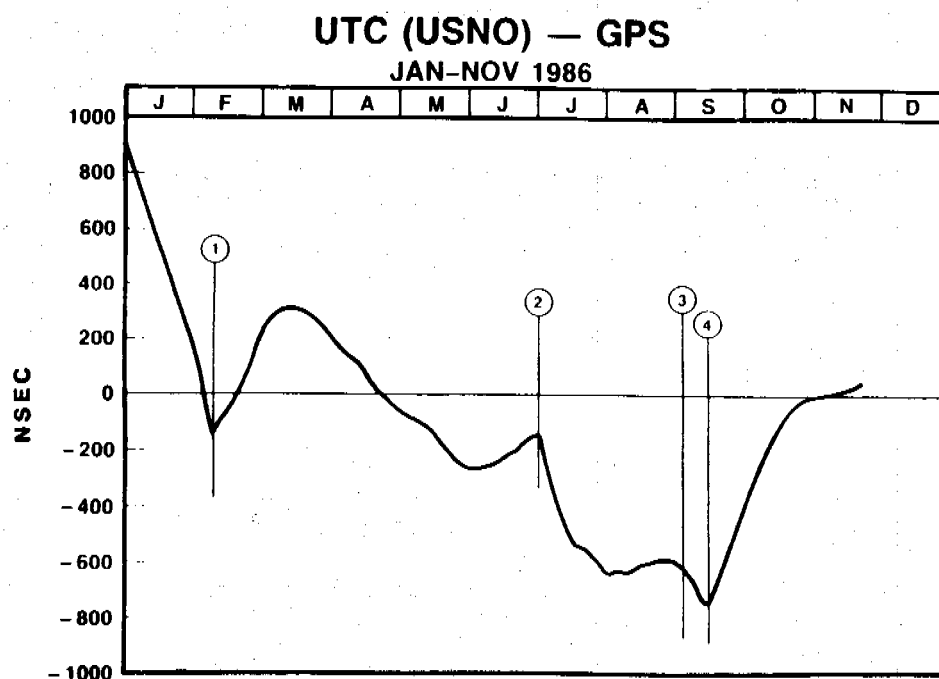
Figure 1 - Differences (in nanoseconds) between UTC(USNO) and GPS Time. Data has been filtered using three day smoothing.
