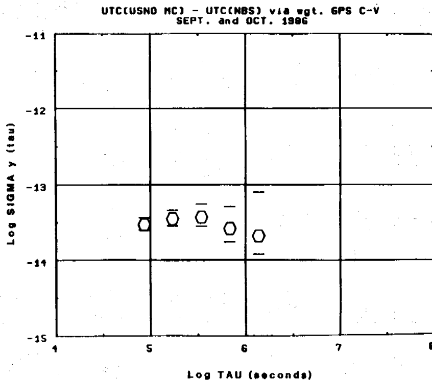
Figure 5 - Measured Frequency Stabilities between UTC(USNO, MC) and UTC(NBS).
