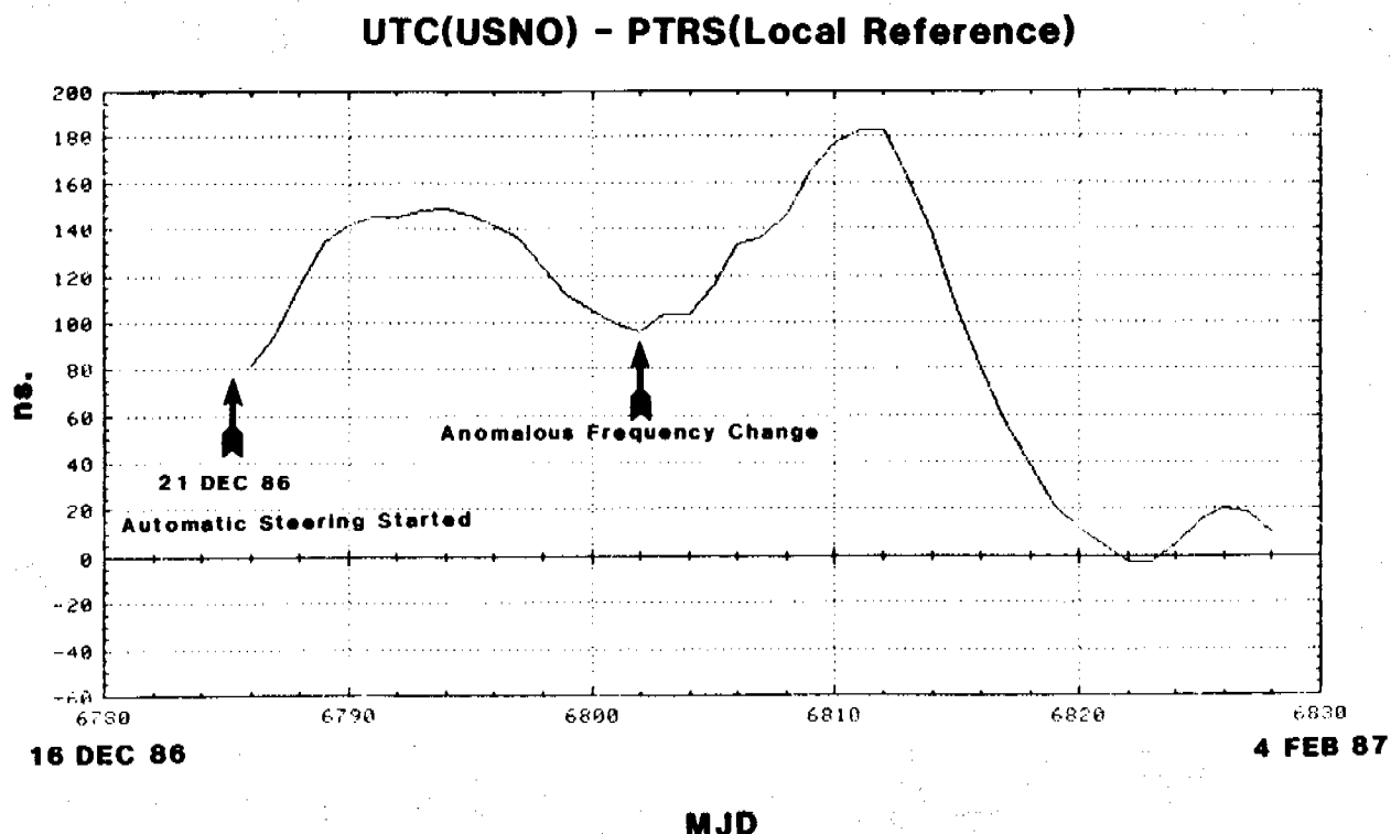
Figure 3 - Differences between UTC(USNO) and the Local Reference Clock of the USNO Precise Time Reference Station (PTRS) in nanoseconds.
