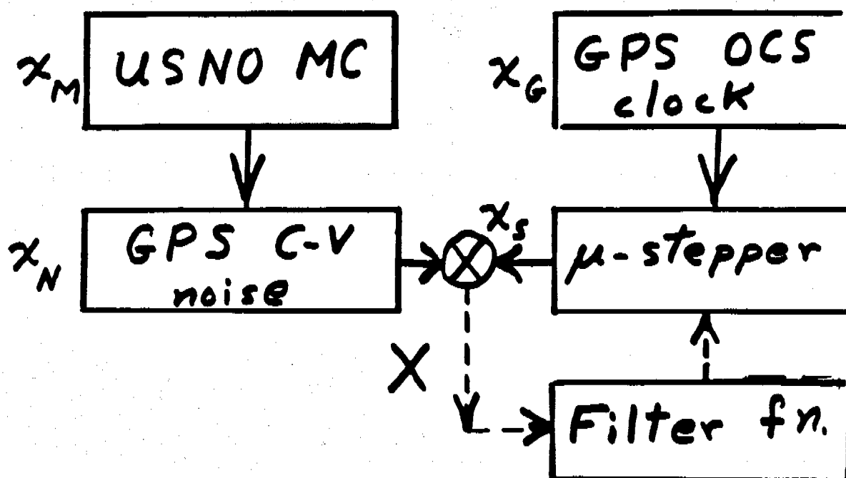
Figure 4 - Block Diagram of the Control Theory Steering Procedures.
