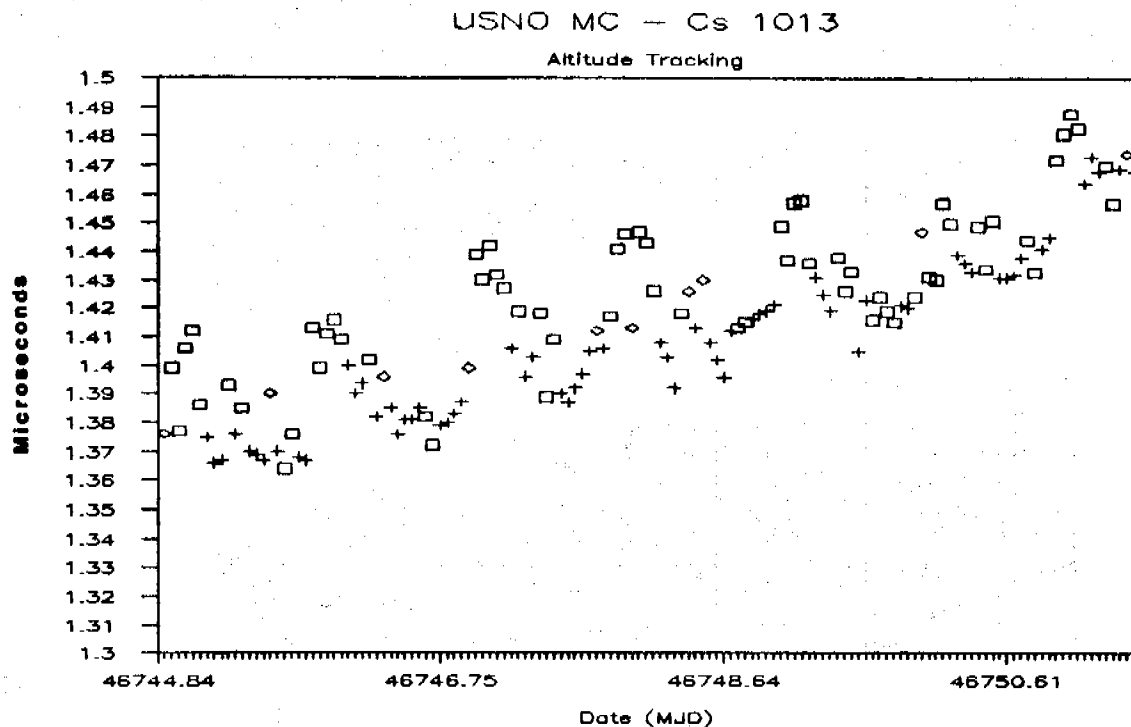
Figure 6 - The square symbols indicate the difference USNO MC - CS 1013 obtained from GPS measurements when satellite elevation was < 45 degrees, while the plus symbols are obtained from tracking GPS satellites when the elevation was > 45 degrees. Diamond symbols are the direct measurements of USNO MC - CS 1013.
