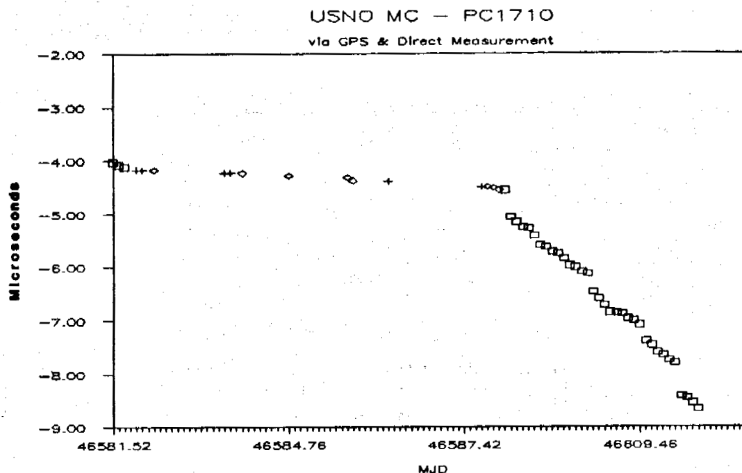
Figure 2 - Square symbols represent measures made at USNO. Plus symbols indicate values obtained using GPS measurements. Measurements of the differences between PC 1449 and PC 1710 were made during this trip. These measurements were used to obtain USNO MC - PC 1710 in the same manner as any other portable clock measurement. These values are represented by the diamond symbols.
