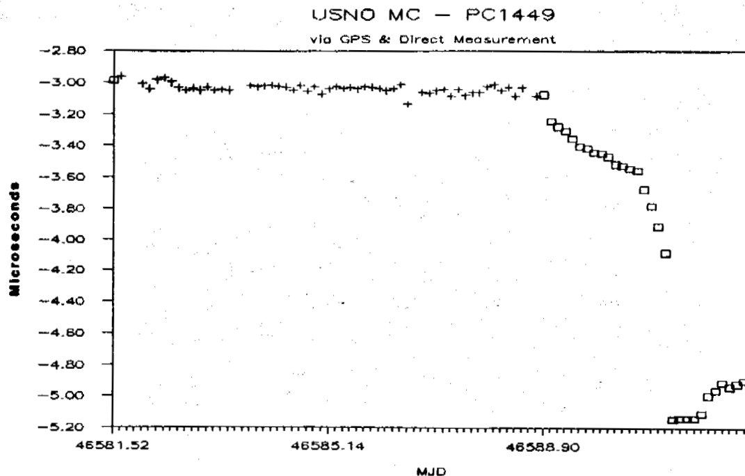
Figure 1 - Square symbols indicate the direct measures made of PC 1449 while at USNO before and after the trip. GPS measures made during the trip were used to obtain values of USNO MC - PC 1449 and are shown by the plus symbols.
