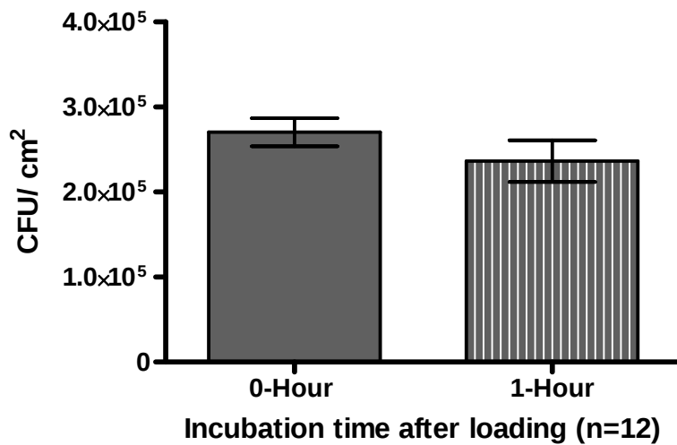
330 Figure 6: Recovery of Staphylococcus aureus loaded onto glass coupons using the Dry 331 Aerosol Deposition Device. Loading time was five minutes.
