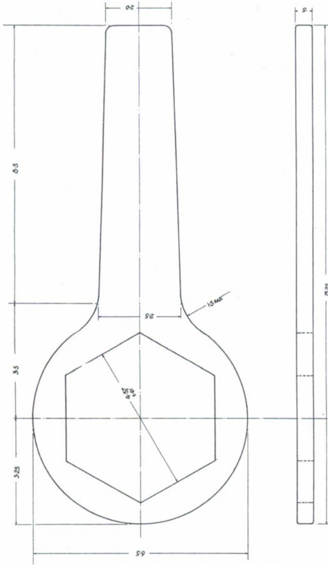
32 1-OFF MILD STEEL - TO FIT DETAILS 2 & 14 OF R.D./C. 303
