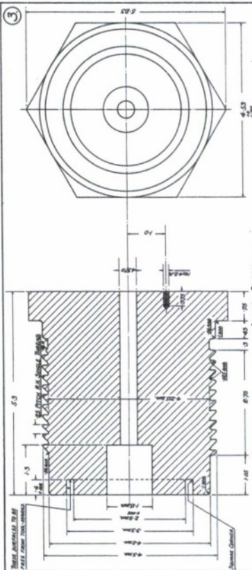
— GAUGE-ELECTRODE BUSH — — L-97. B.S. AUTO. 500S/40 (OR EQUIVALENT) HEAT-TREATED TO 45 TON/50 N. YIELD —
