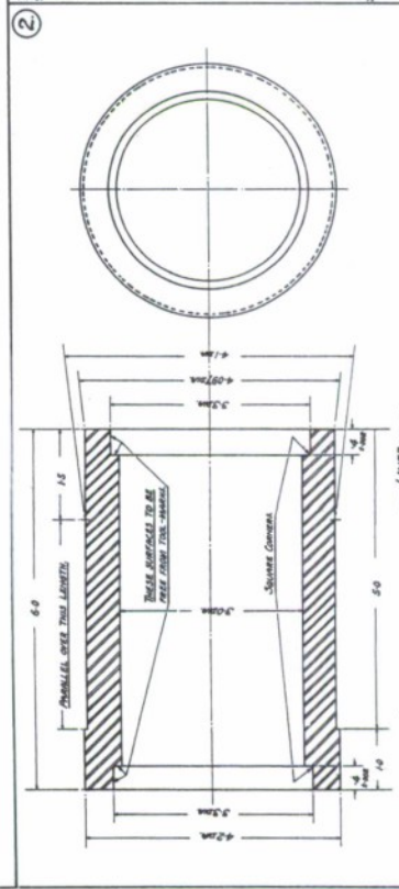
— LINER — — L-97. HYDRO. 30 (OR EQUIVALENT) HEAT-TREATED TO 55 TON/50 N. YIELD —
