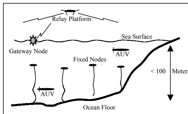
Fig. 1 Nominal Underwater Acoustic Network
