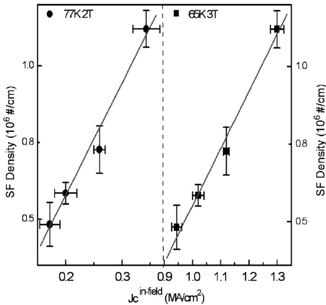
FIG. 3. The plot of SF density as a function of J_c^{\text{in-field}} ( H\parallel c ) at 65 K, 3 T and at 77 K, 2 T for the samples on STO substrate. A clear linear relation is observed between the SF density and the J_c^{\text{in-field}} .
