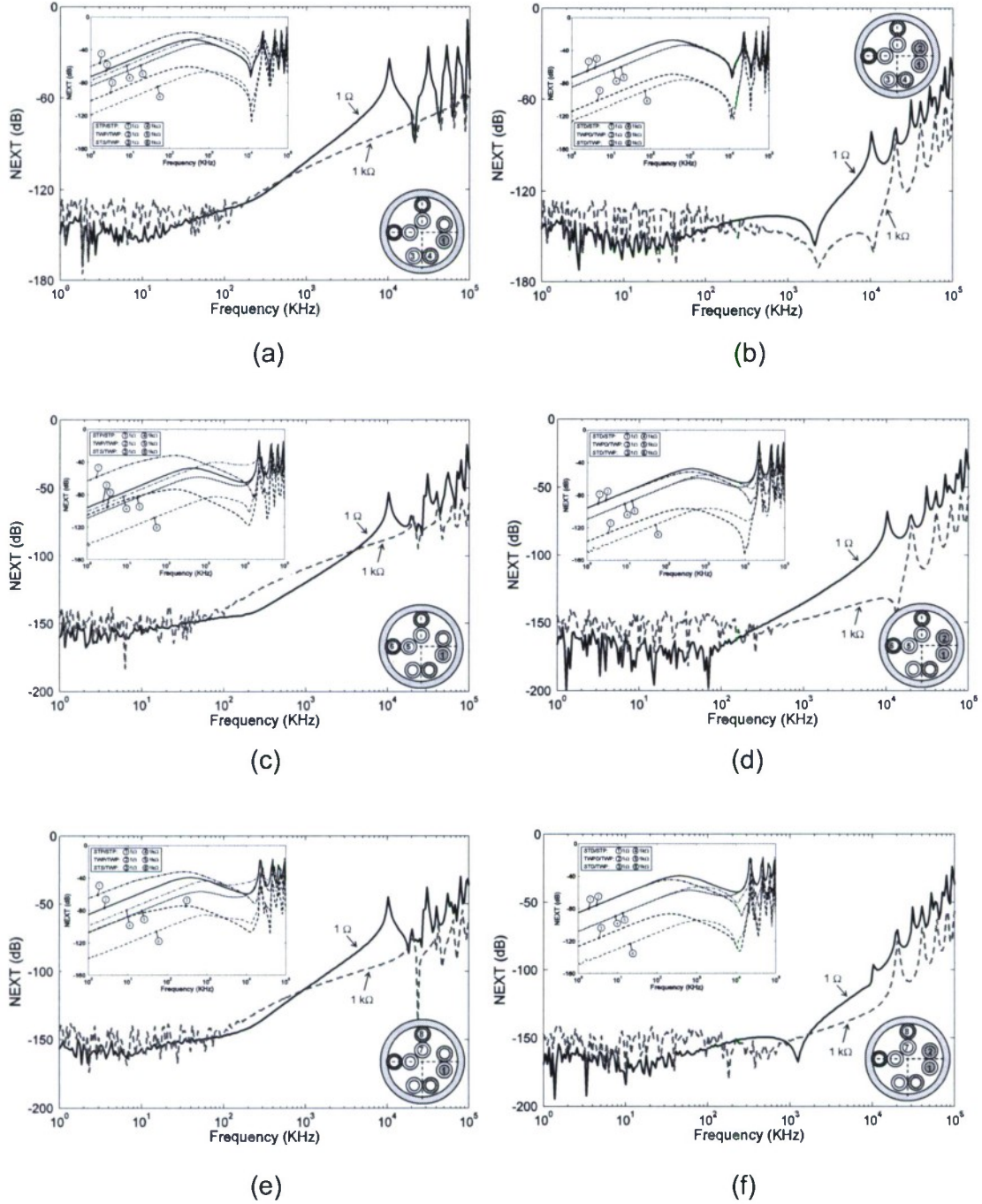
Fig. IVB-4 NEXT levels across Conductors 3-4 ((a) and (b)), Conductors 5-6 ((c) and (d)), and Conductors 7-8 ((e) and (f)) as functions of the source and load impedances (1 \Omega and 1 k \Omega ) in the frequency domain for coupling circuits driven by a +0.5 V source on conductor 1 and \pm 0.5 V sources on Conductors 1 and 2. The plots shown in the inset are the results using different crosstalk models from the previous study [22].
